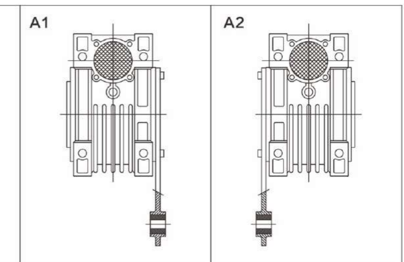
扭力臂配置 Position of torque arm
