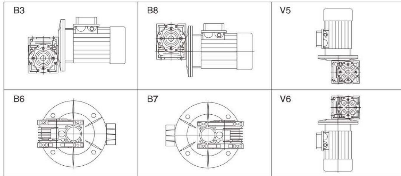
单级安装型式 Single Step Mounting Positions
